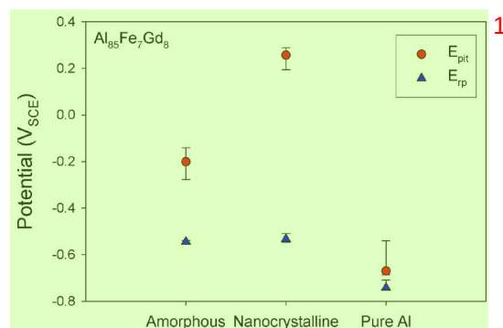
Figure 8. (Color online) Median pitting and repassivation potentials for \text{Al}_{85}\text{Fe}_7\text{Gd}_8 and pure Al in deaerated 0.6 M NaCl. Error bars represent the 25th and 75th percentile of the data. Scan rate 0.1 mV/s.
