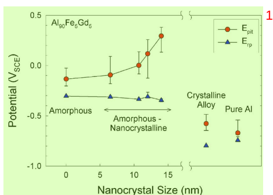
Figure 5. (Color online) Median pitting and repassivation potentials for \text{Al}_{90}\text{Fe}_5\text{Gd}_5 and pure Al in deaerated 0.6 M NaCl. Error bars represent the 25th and 75th percentile of the data when expressed as the cumulative probability of obtaining the given pitting potential. Scan rate 0.1 mV/s.
