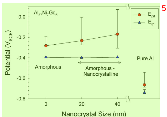
Figure 6. (Color online) Median pitting and repassivation potentials for \text{Al}_{87}\text{Ni}_7\text{Gd}_6 and pure Al in deaerated 0.6 M NaCl. Error bars represent the 25th and 75th percentile of the data. Scan rate 0.1 mV/s.
