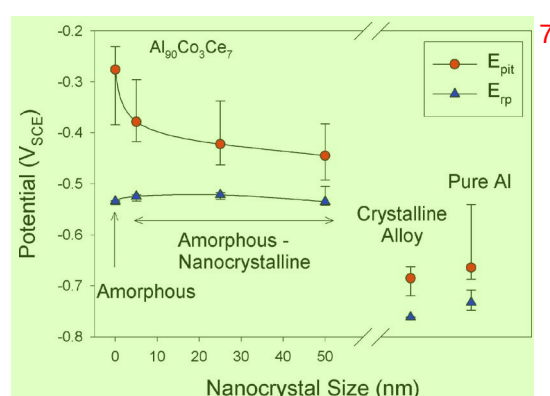
Figure 7. (Color online) Median pitting and repassivation potentials for \text{Al}_{90}\text{Co}_3\text{Ce}_7 and pure Al in deaerated 0.6 M NaCl. Error bars represent the 25th and 75th percentile of the data. Scan rate 0.1 mV/s.
